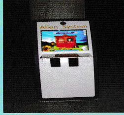
Alien System
