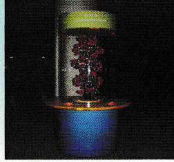
DNA Composition
