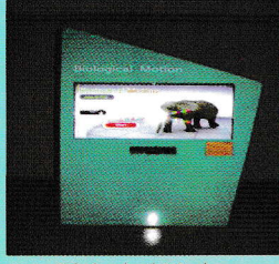
Biological Motion
